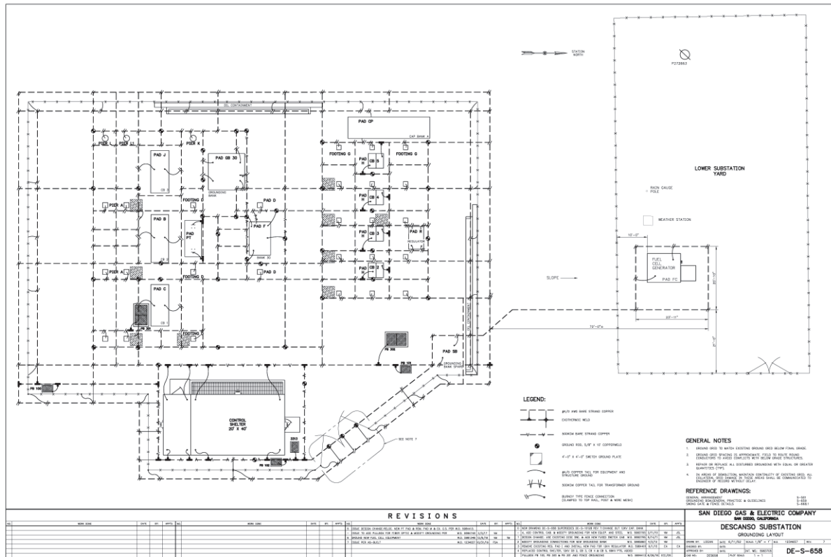
Figure 2-1. SDG&E Grounding Layout for Descanso Substation
