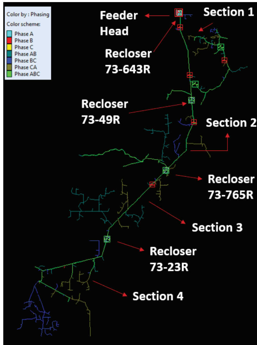
Figure 4-2. Synergi Model of Circuit 73: Individual Sections and Reclosers are Labelled Separately
