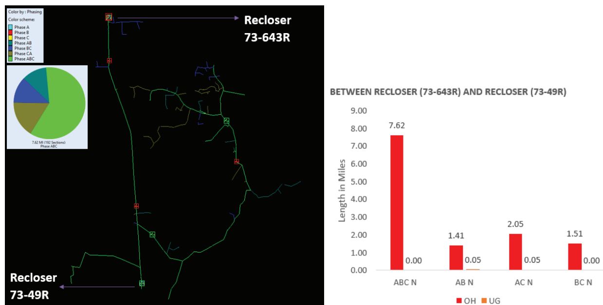
Figure 4-10. Synergi Model of Section 1 of C73 Showing Phasing of Conductors with Their Respective Length
