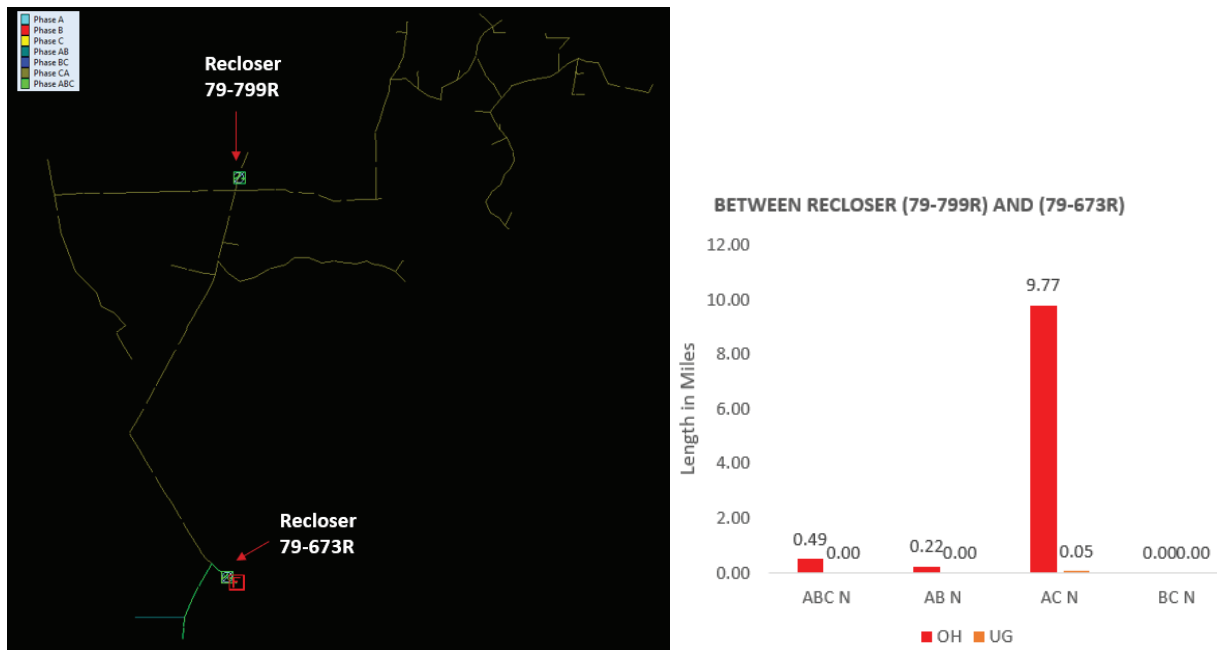
Figure 4-21. Synergi Model of Section 9W of C79 Showing Phasing of Conductors with Their Respective Length
