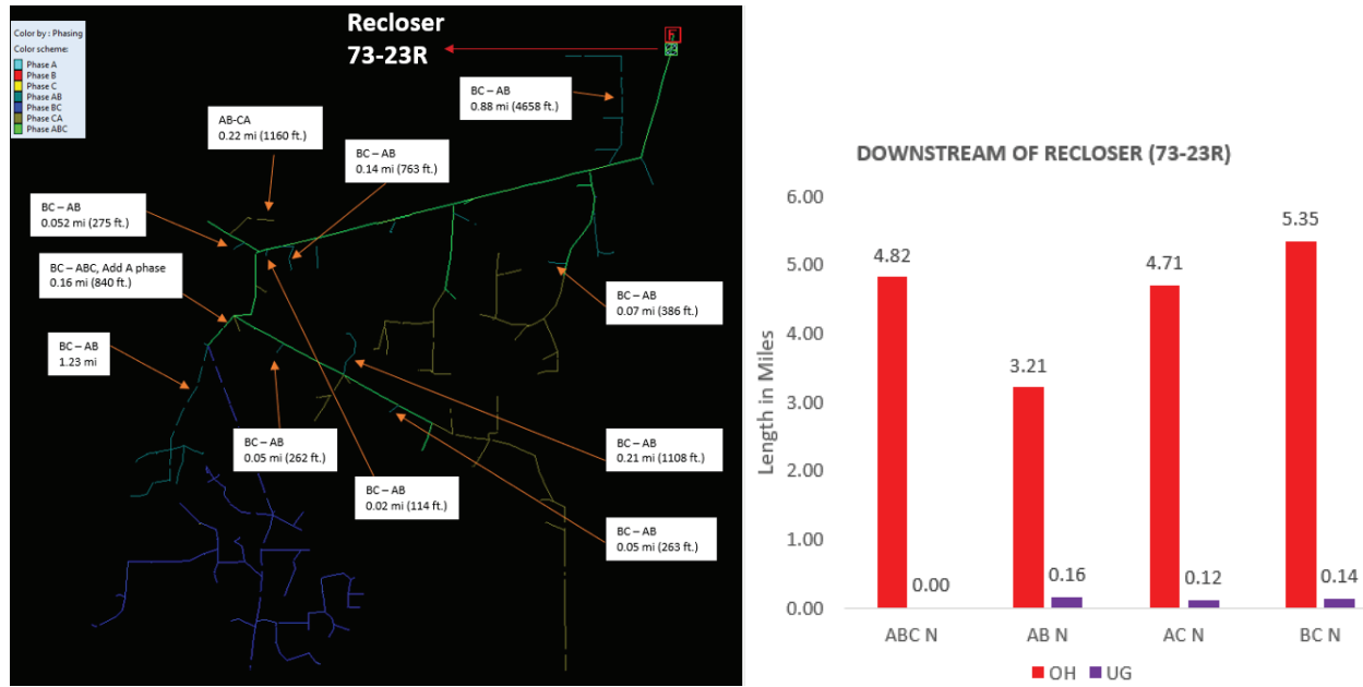
Figure 4-35. Phase Swaps and Additional Conductor on Section 4 of C73
