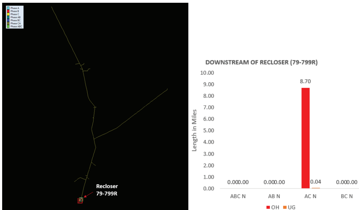
Figure 4-22. Synergi Model of Section 10W of C79 Showing Phasing of Conductors with Their Respective Length
