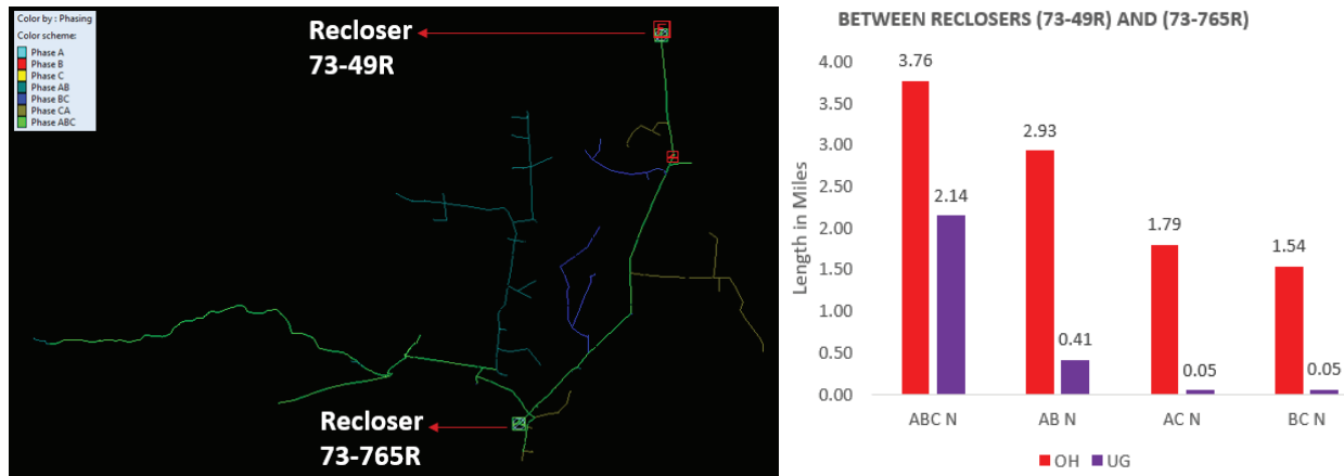
Figure 4-9. Synergi Model of Section 2 of C73 Showing Phasing of Conductors with Their Respective Length
