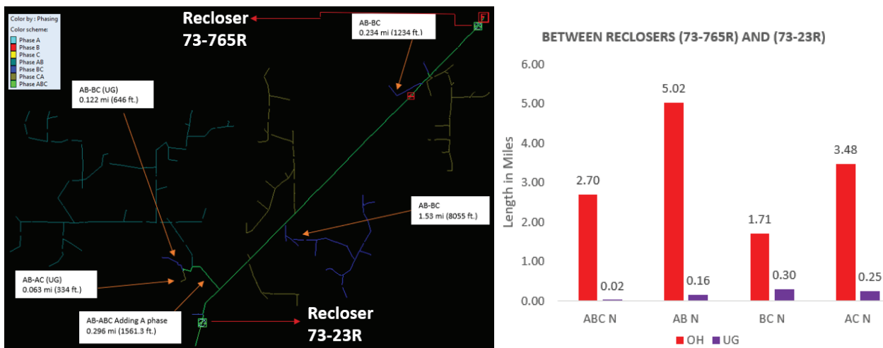
Figure 4-36. Phase Swaps and Additional Conductor on Section 3 of C73
