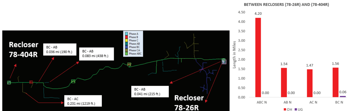
Figure 4-29. Section 1 Phase Swaps on C78
