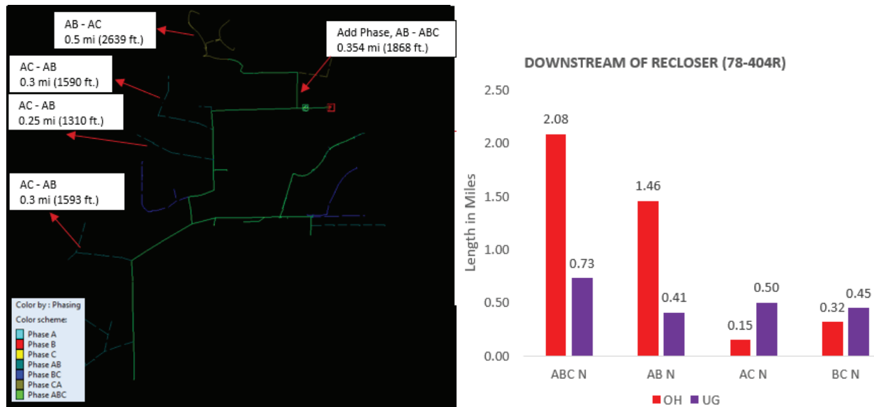
Figure 4-37. Phase Swaps and Additional Conductor on Section 2 of C78
