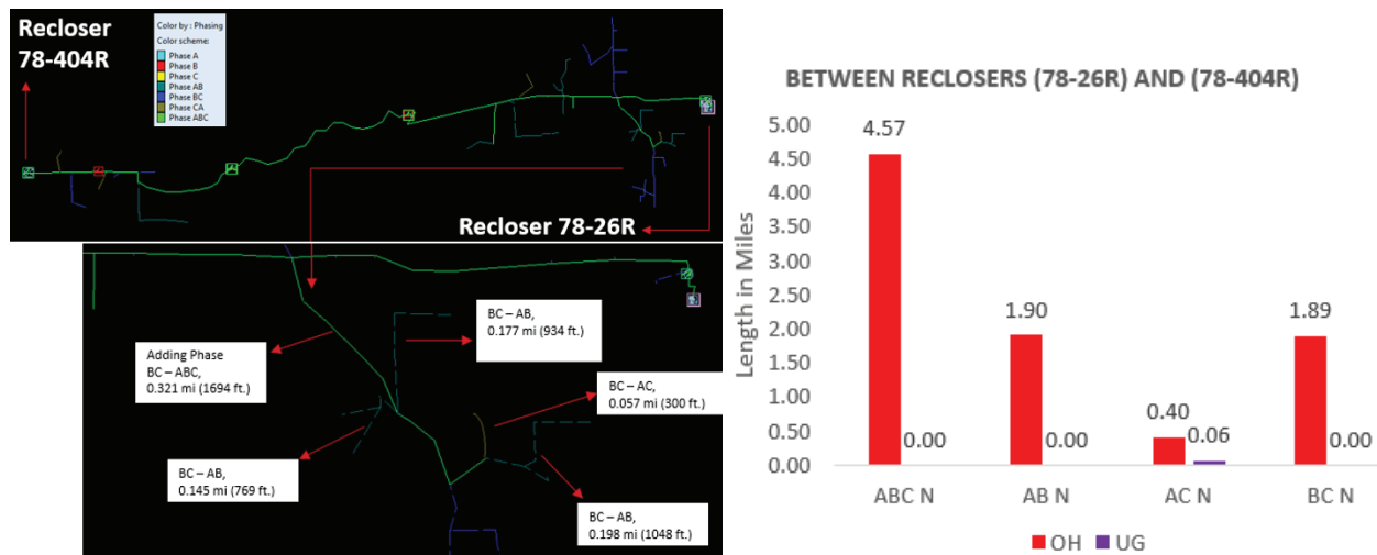
Figure 4-38. Phase Swaps and Additional Conductor on Section 1 of C78
