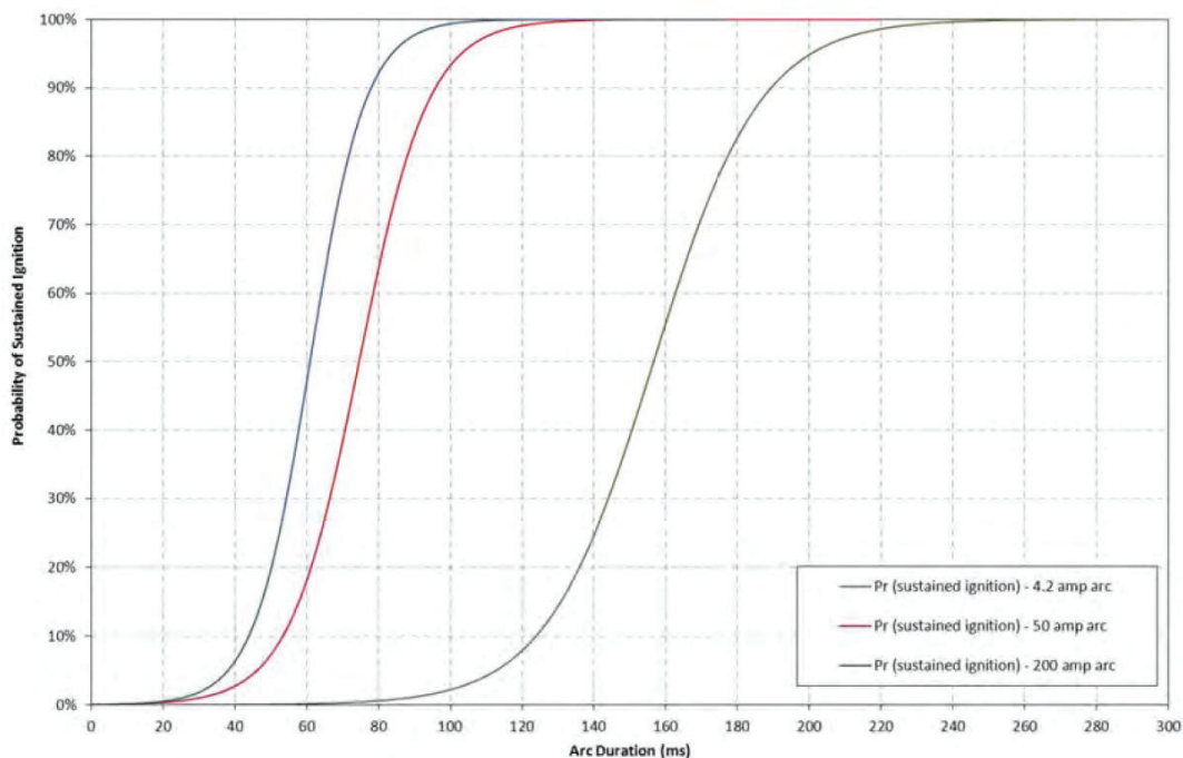
Figure 7-1. Probability of Sustained Ignition in Function of Time and Fault Current
